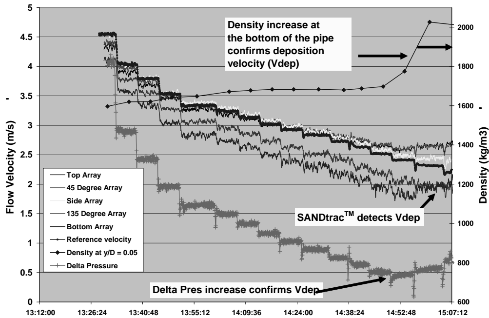
Figure 9: 186 \mu\text{m} Slurry solid deposition detected by sonar meter, densitometer, and delta-pressure
