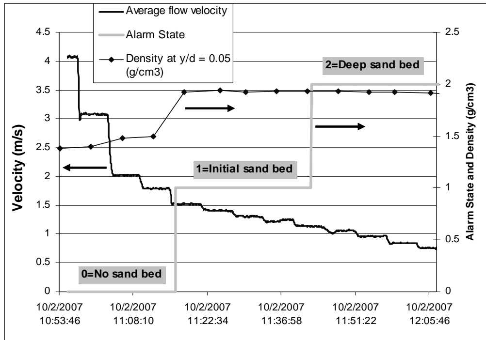
Figure 6: Alarm States– 89 \mu\text{m} slurry.
