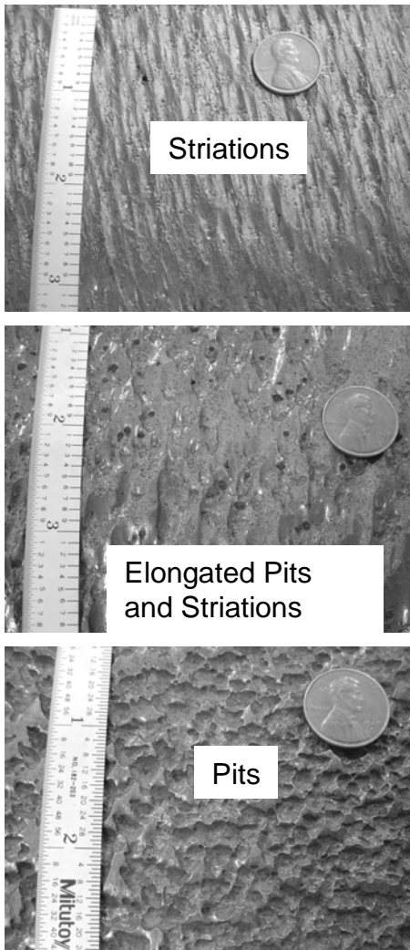
Figure 21: Inner surface irregularities seen on chromium-steel worn pipe
