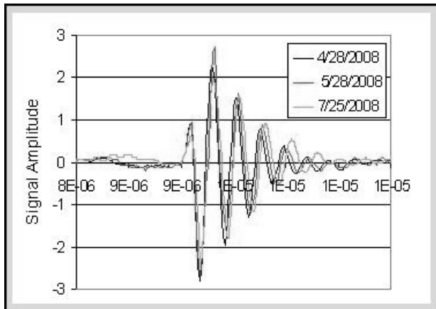
Figure 23: Long Term High Temperature Testing
