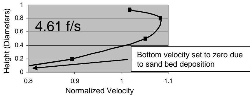
Figure 8: Heterogeneous flow, stationary solids bed
