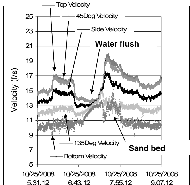
Figure 14 Detection of water flush (no stratification) and sand bed deposition in slurry pipeline in the field
