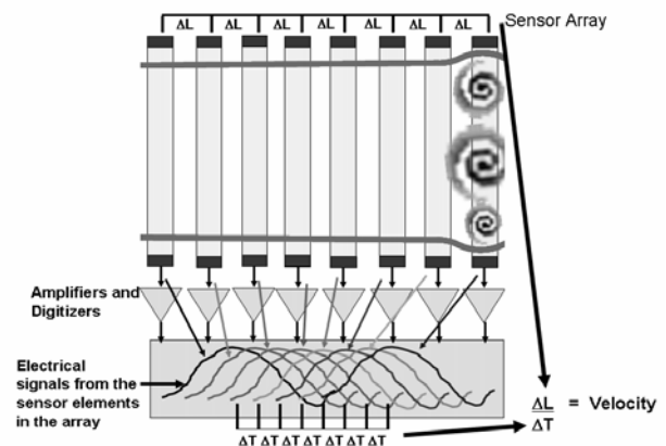
Figure 2. Illustration of signal detected by passive sensors in array from one collection of turbulent eddies
