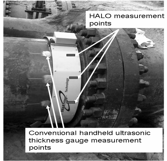
Figure 16: Pipe wall thickness measurement points to compare conventional technique with HALO™
