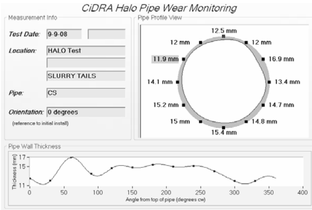
Figure 18: HALO™ pipe wall thickness visualization software output
