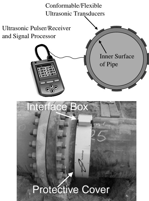
Figure 15: Conceptual layout of HALO™ system and picture of system in operation at a customer site
