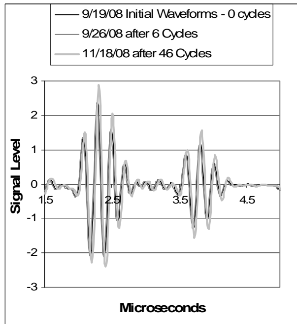
Figure 22: Impact of Temperature Cycling on Wall Thickness Measurement and Signal Amplitude (-40C to +40C with 10 hour holds)
