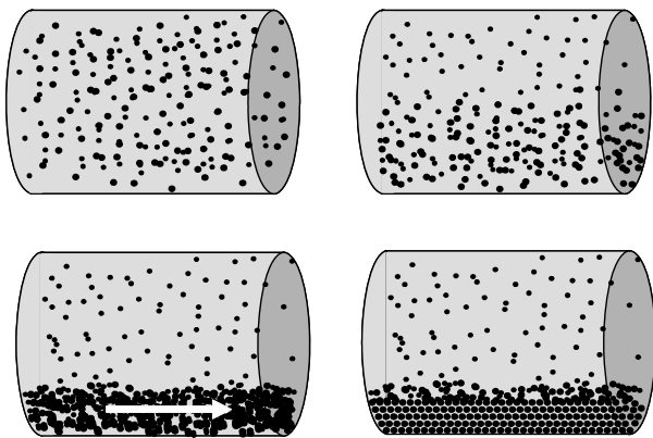
Figure 3 (Top Left) Homogeneous flow (Top Right) Heterogeneous flow – full suspended particles (Bottom Left) Heterogeneous flow – moving bed (Bottom Right) Heterogeneous flow – stationary bed
