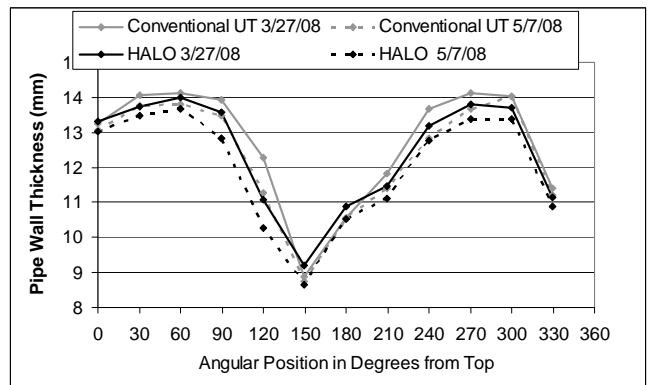
Figure 17: Conventional ultrasonic (UT) pipe wall thickness measurement versus HALO™ measurements
