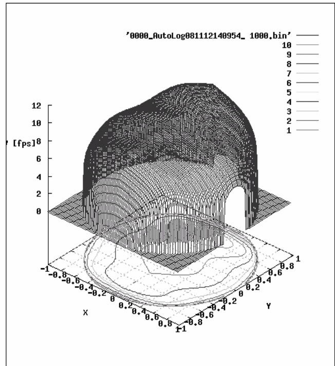
Figure 11: Three-dimensional velocity profiles and velocity contours in an inhomogeneous flow
