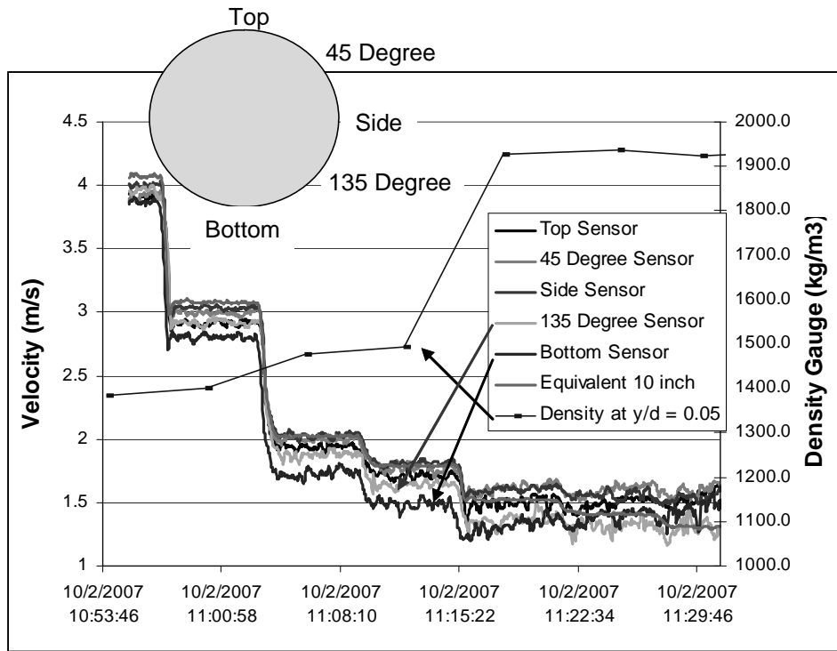
Figure 5: Velocity profile of 89 \mu\text{m} mining slurry.
