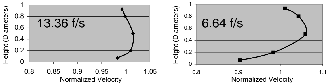
Figure 7: (Left) Mostly homogenous flow, suspended particles and (Right) Heterogeneous flow, suspended particles
