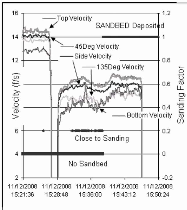
Figure 13 Detection of sand bed and development of sand bed in slurry pipeline in the field
