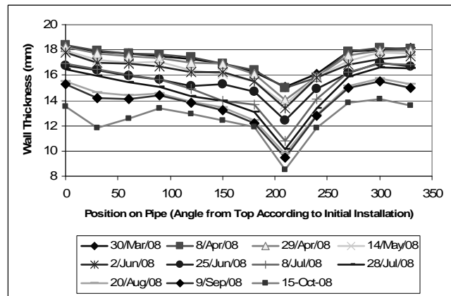
Figure 20: Measurement of pipe wall thickness as a function of angular position and time is shown
