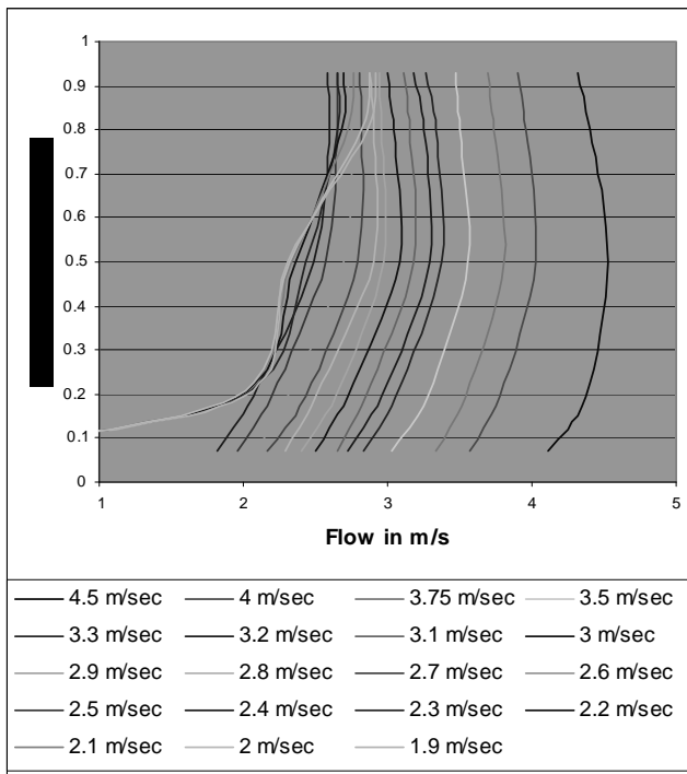
Figure 10: Velocity profiles vs. reference velocity
