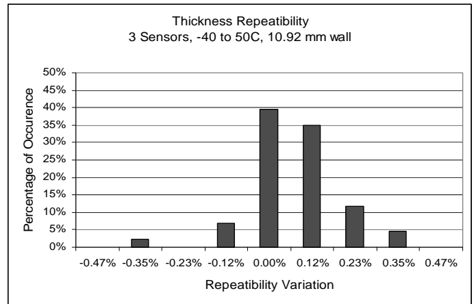
Figure 19: Small spread in data over 90C temperature range and over three sensors is shown
