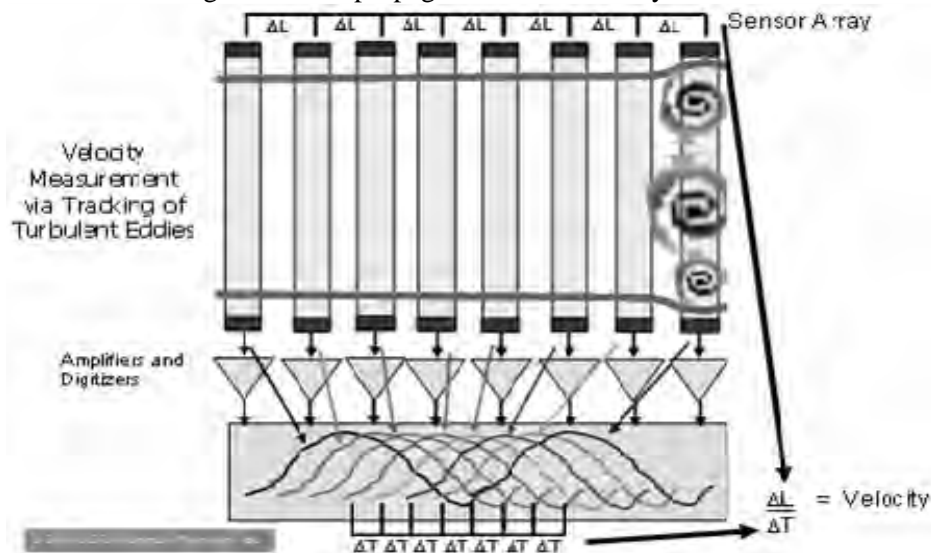
Figure 1: Basic operating principle. Tracking velocity of vorticle pressure fields straining pipe wall.
