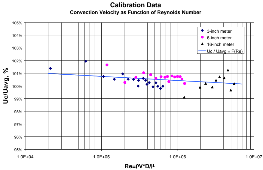
Figure 4: Ratio of convection velocity to volumetrically-averaged flow rate as function of Reynolds Number for 3", 6", and 16 " Sonar-based flow meters
