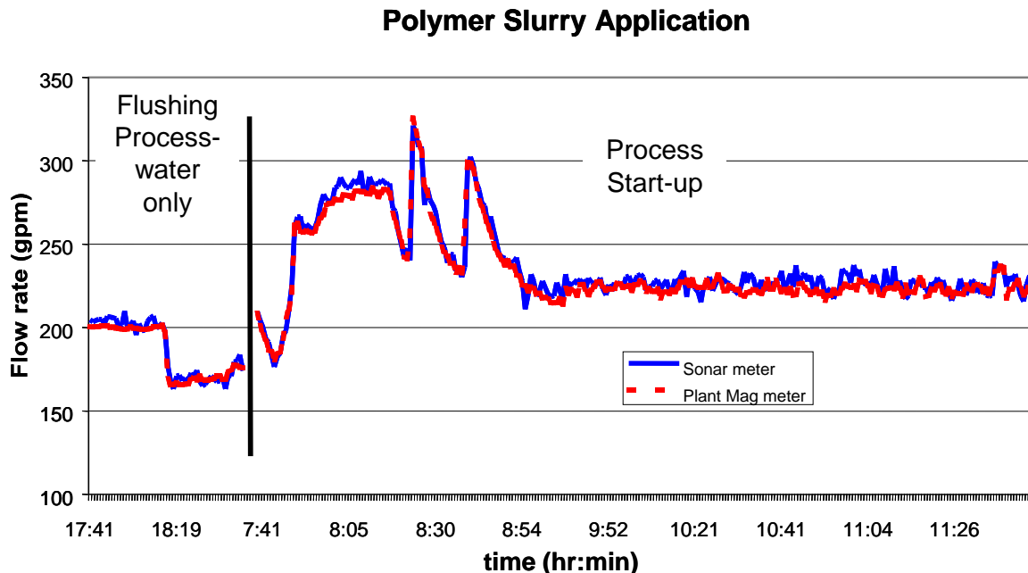
Figure 8: Comparison of Sonar-Based Flow meter with Electromagnetic flow meter on a liquid-conveyed, solid-particle slurry
