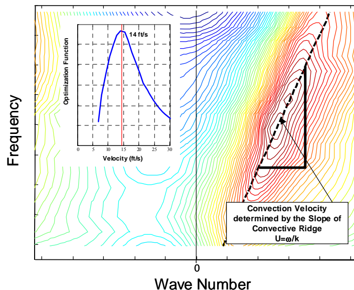
Figure 2: K- \omega plot generated from an array of sensors listening to water flowing in a 6 inch pipe at ~1000gpm.
