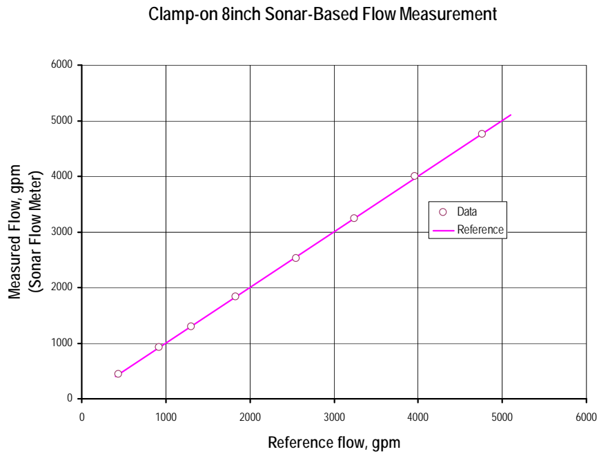
Figure 7: Volumetric Flow Rate measured using the Sonar based flow meter versus Reference Flow Rate
