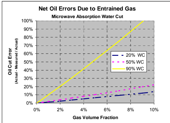
Figure 3: Effect of Free Gas on Interpreted Oil Cut Using Microwave Absorption Devices
