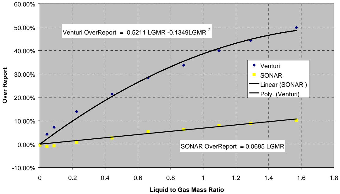
Figure 8: Over-report data as a function of wetness at a nominal flow rate of 40 ft/sec at 200 psi (Froude number = 1.5)
