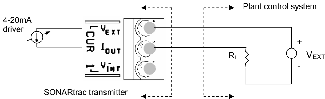
Figure 1 Externally Powered 4-20mA Loop
