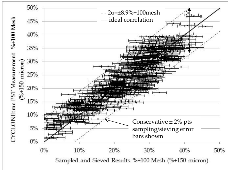
Figure 2 CYCLONetrac PST 150 micron measurements compared to the sieved samples for a copper/molybdenum concentrator processing copper porphyry ore
