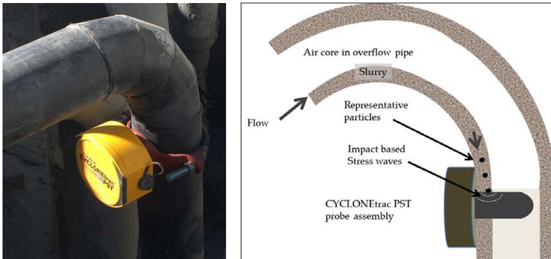
Figure 1 CYCLONEtrac PST installed on overflow pipe (left); illustration of principle of operation (right).
