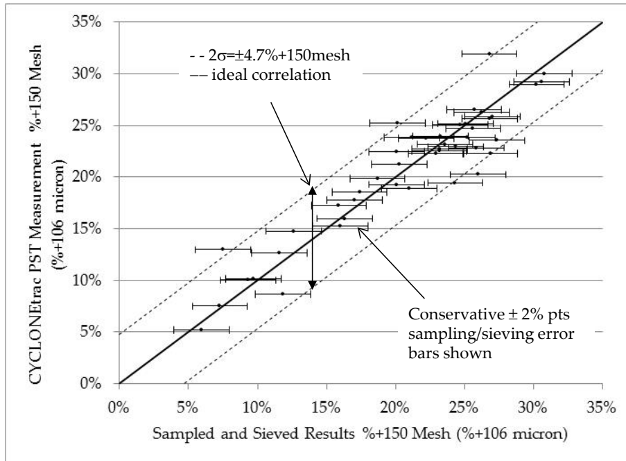
Figure 8 CYCLONetrac PST 106 micron measurements compared to the sieved samples for a gold concentrator
