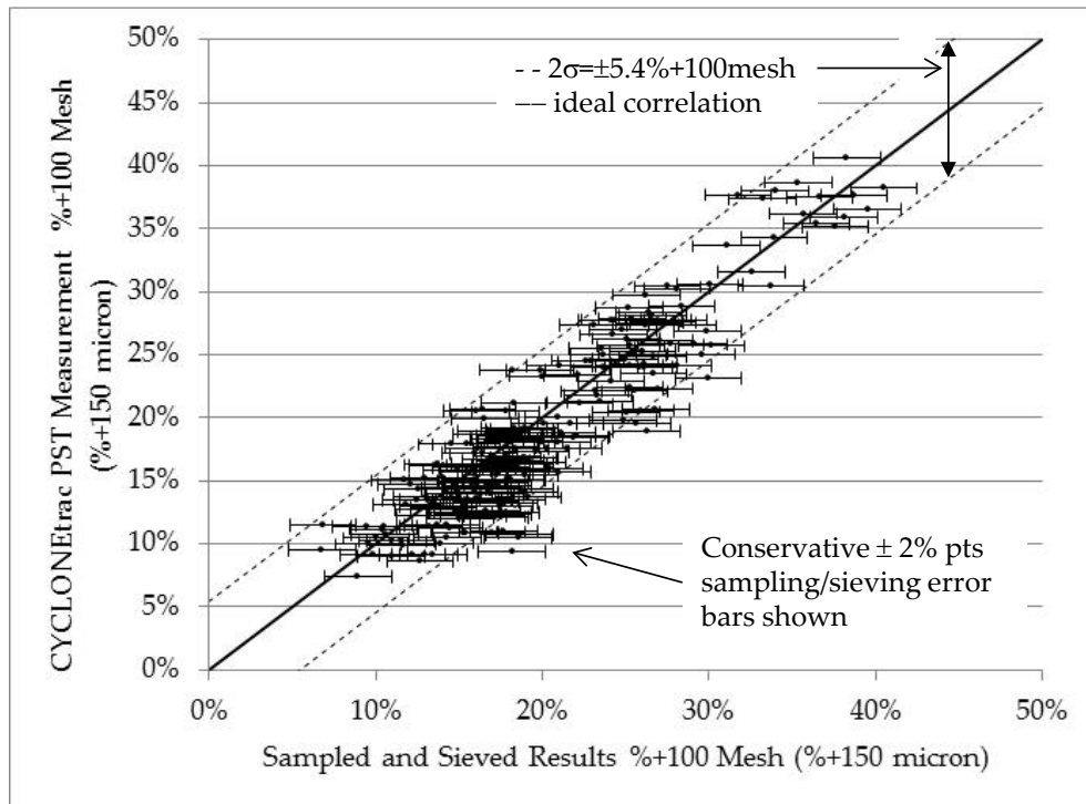
Figure 4 CYCLONetrac PST 150 micron measurements compared to the sieved samples for a large copper concentrator
