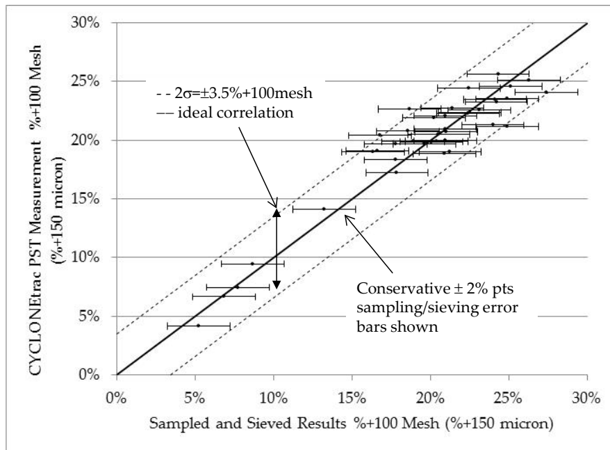
Figure 7 CYCLONetrac PST 150 \mu m measurements compared to the sieved samples for a phosphate plant
