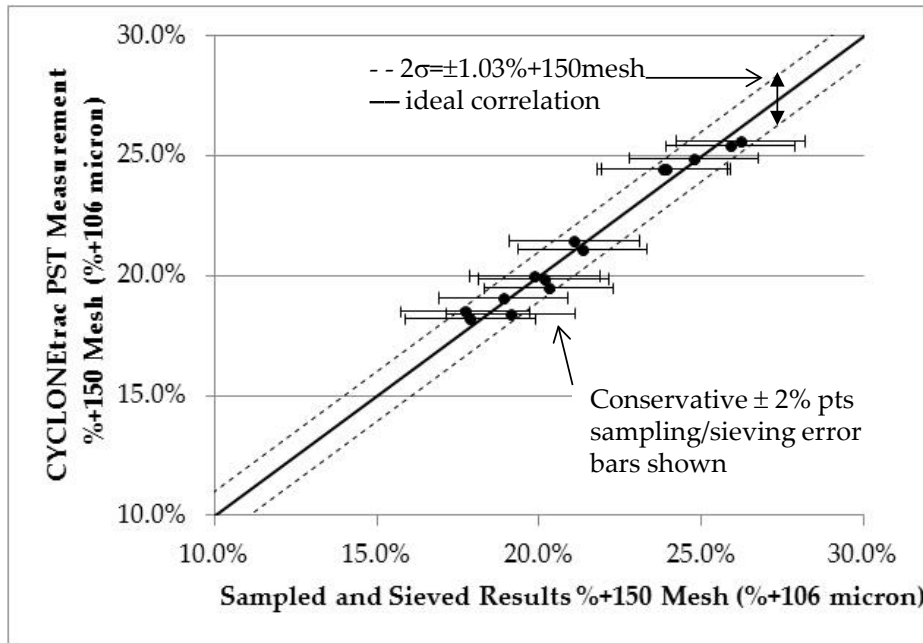
Figure 5 CYCLONEtrac PST 74 micron measurements compared to the sieved samples for an iron ore concentrator
