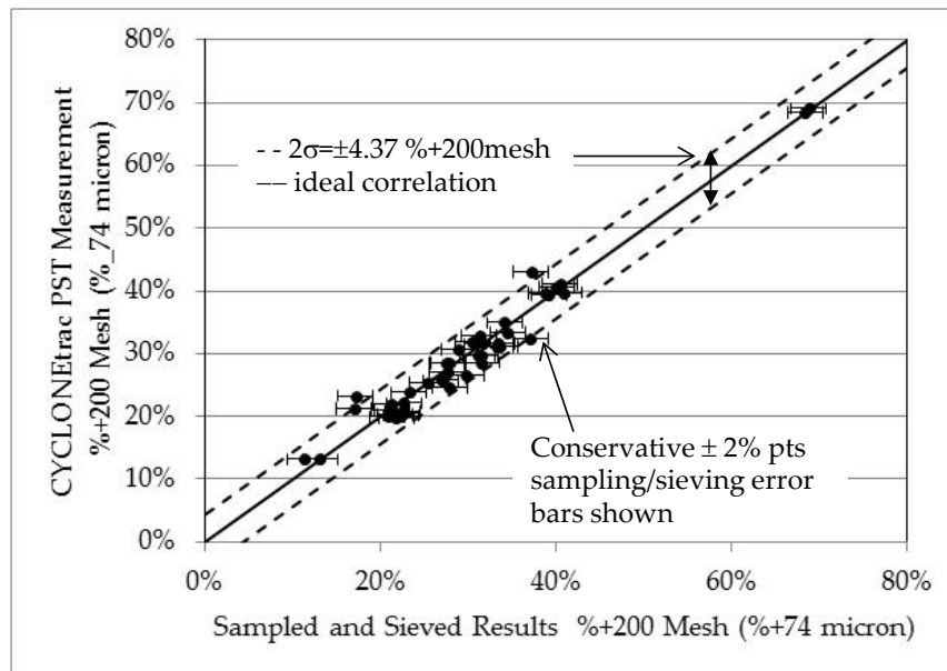
Figure 3 CYCLONEtrac PST 74 micron measurements compared to the sieved samples for a copper, silver and gold plant dominated by silica and feldspar in the ore
