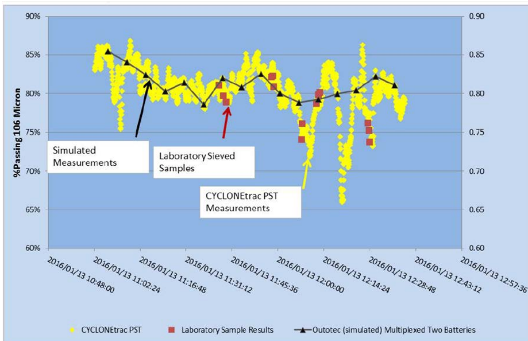
Figure 9 Comparison of PST signal at four second update rate with simulated multiplexed caliper system with six minute update rate, plus manual samples
