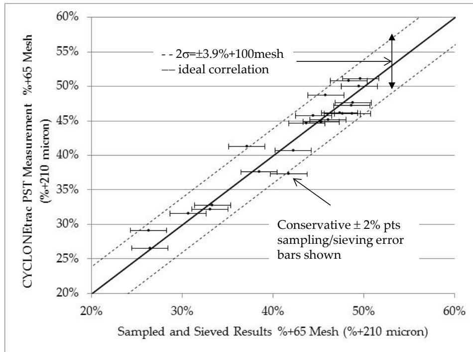
Figure 6 CYCLONetrac PST 210 μm measurements compared to the sieved samples for a coppery/molybdenum plant
